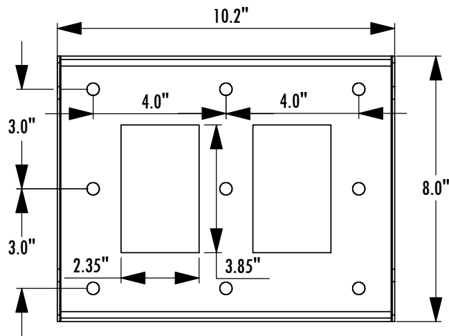
LC200WT Back Plate
