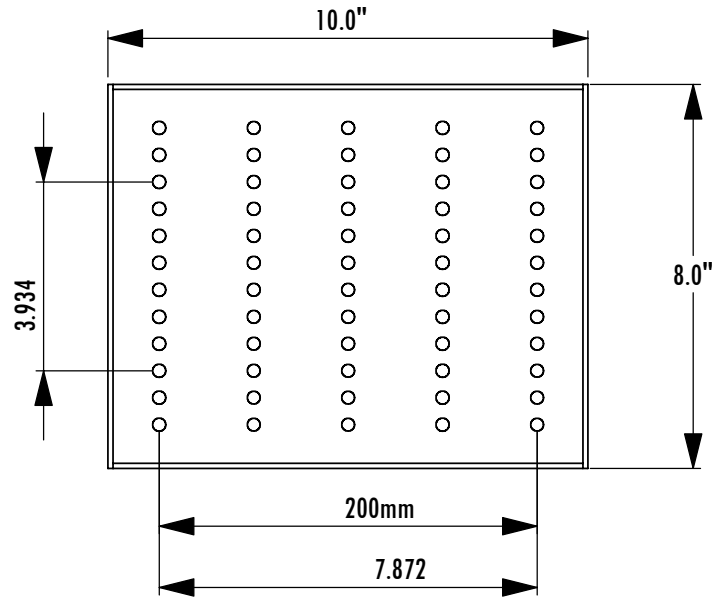
LC200WT VESA® Front
