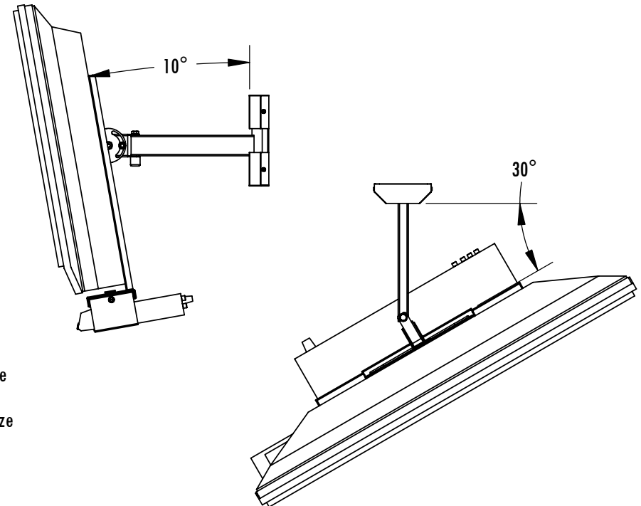
LC200WA2 with LCAPDVD2 Side View Tilt
