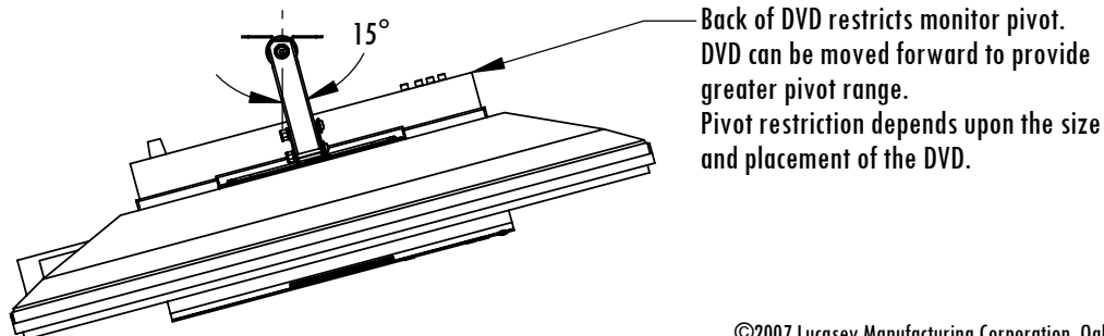
LC100WP or LC200WP with LCAPDVD2 Top View Pivot
